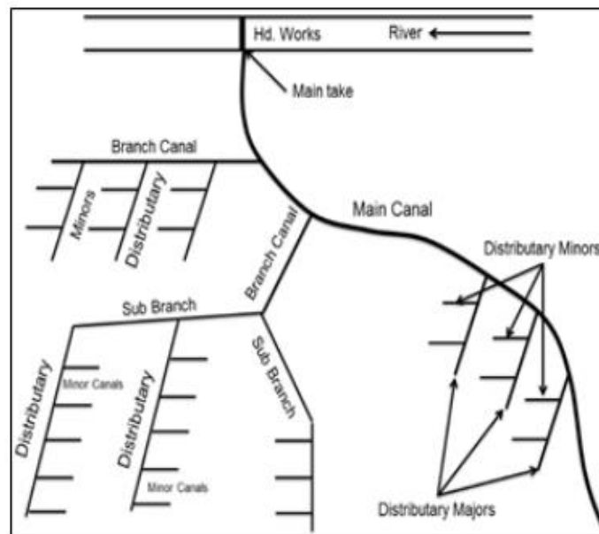
Fig. 8. Typical suitable irrigation network
